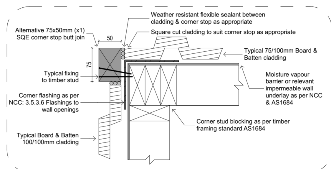
2.1 BB04:B1 - Board & Batten Alternate External Corner Details 1:5
