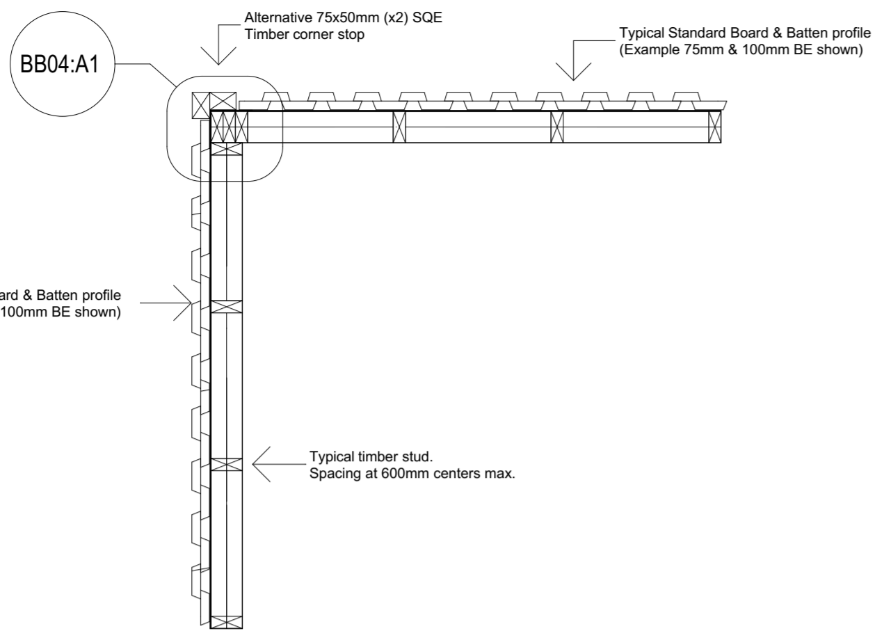
1.0 BB04:A - Typical Board & Batten External Corner 1:15
