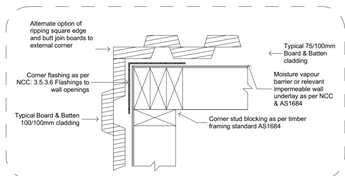
1.2 BB04:A2 - Board & Batten Alternate External Corner Details 1:5
