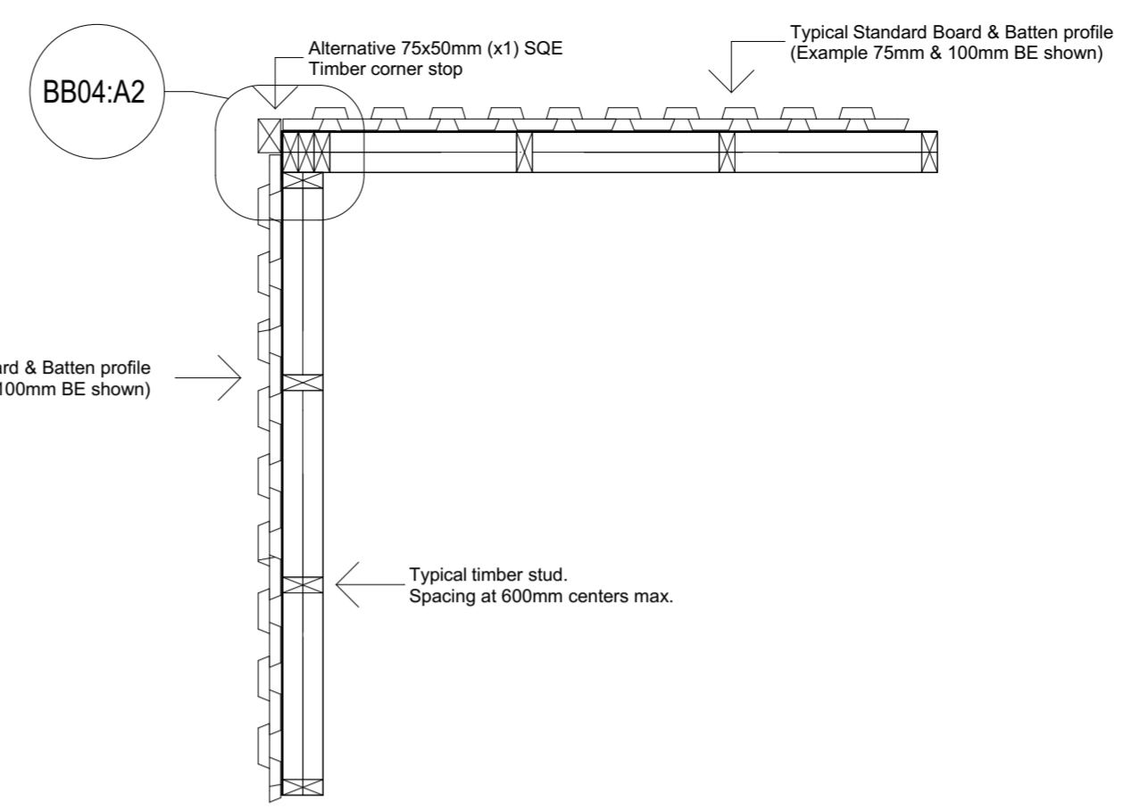
2.0 BB04:B - Alternate Board & Batten External Corner 1:15
