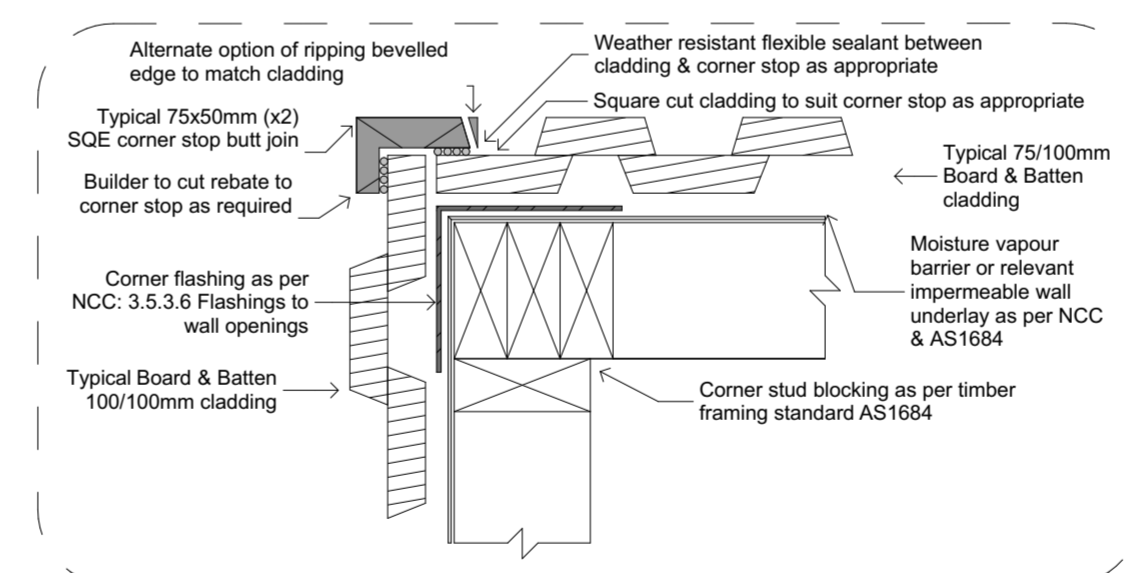
2.2 BB04:B2 - Board & Batten Alternate External Corner Details 1:5
