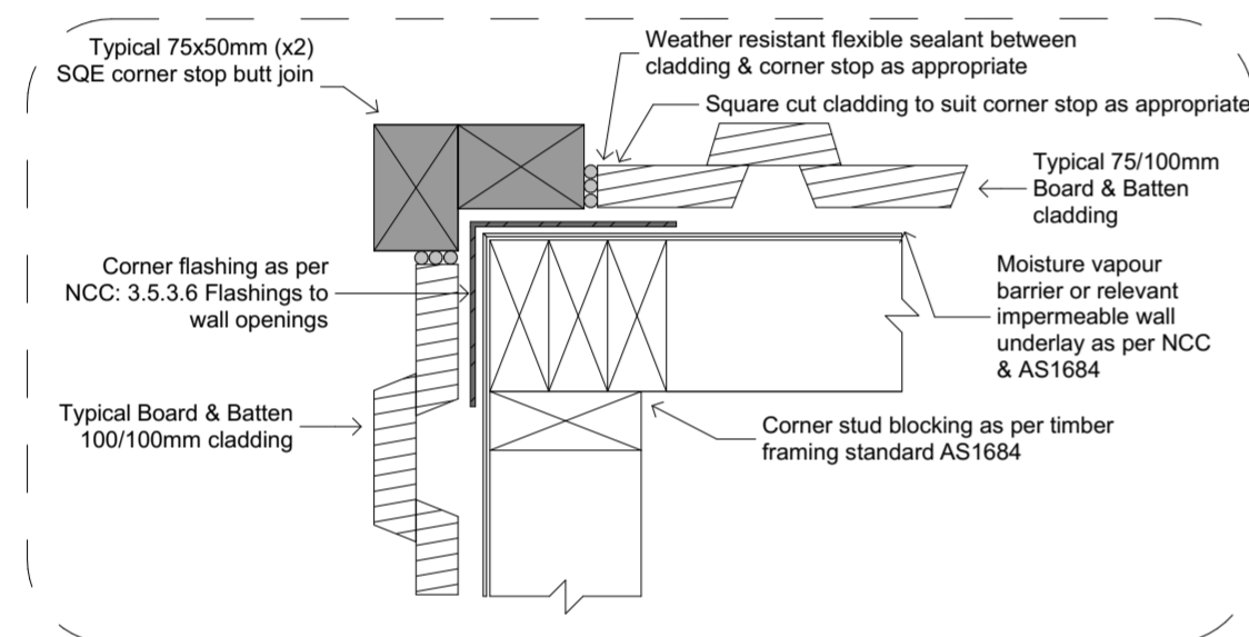
1.1 BB04:A1 - Board & Batten External Corner Details 1:5
