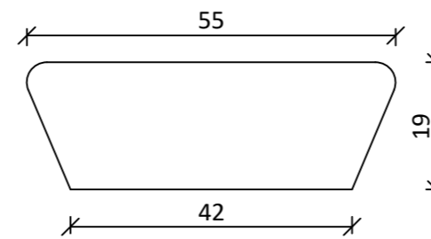
Radial Deck (RSB19055SA) 55 x 19mm
