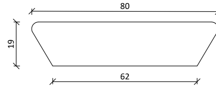
Radial Deck (RSB19080SA) 80 x 19mm
