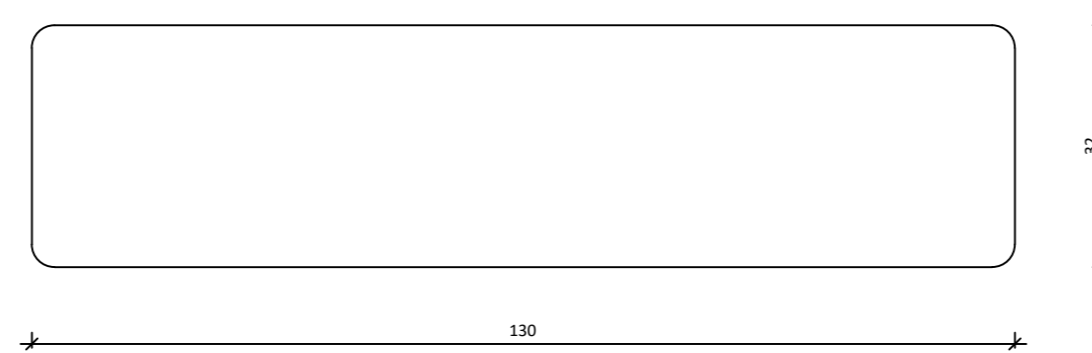
Radial Boardwalk Decking Board (CDB32130SA) 130 x 32mm
