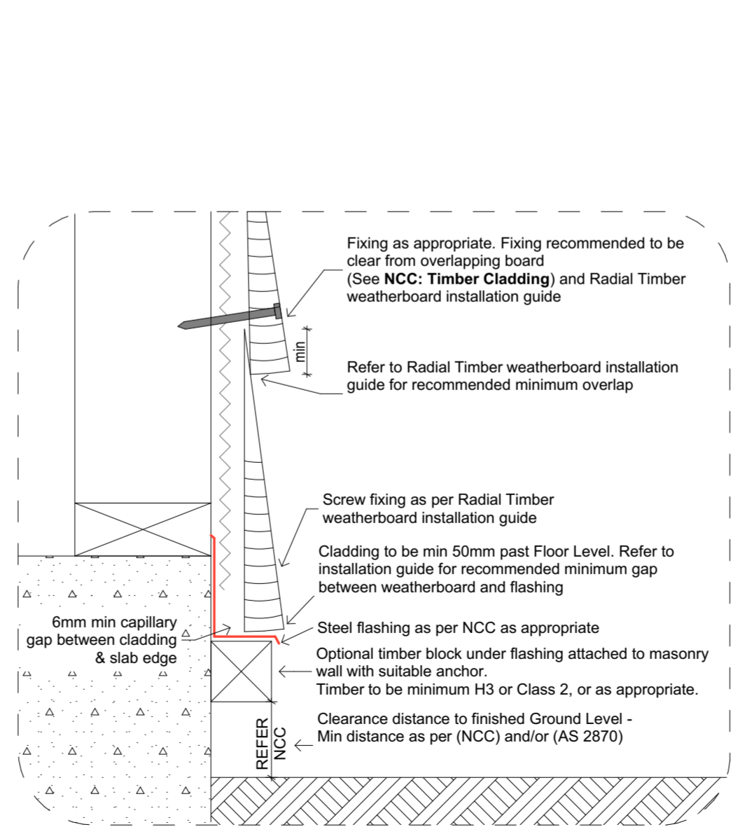
2.1 NE02:B1 - Radial Natural Edge Weatherboard SOG - Bottom Flashing
