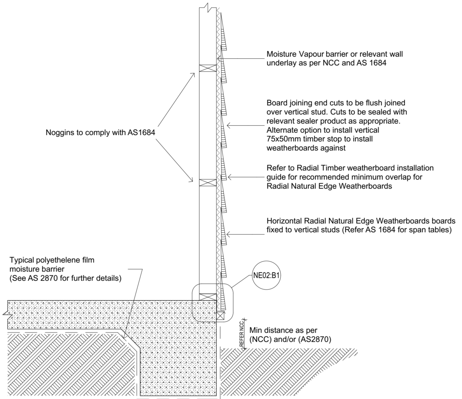
2.0 NE02:B - Horizontal Radial Natural Edge Weatherboard - Stud Frame: SOG
