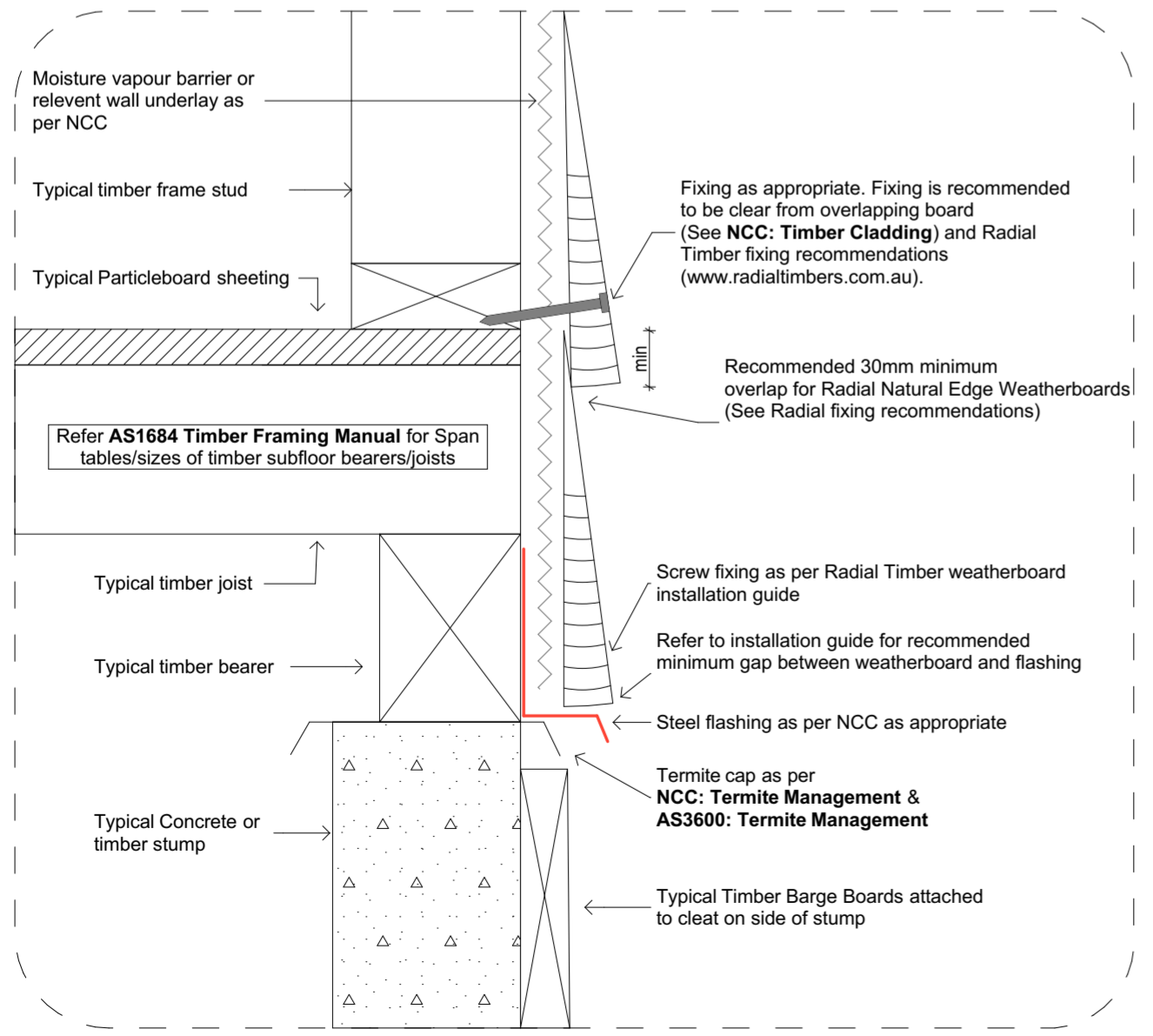
1.1 NE02:A1 - Radial Natural Edge Weatherboard - Bottom Flashing - Timber SubFloor
