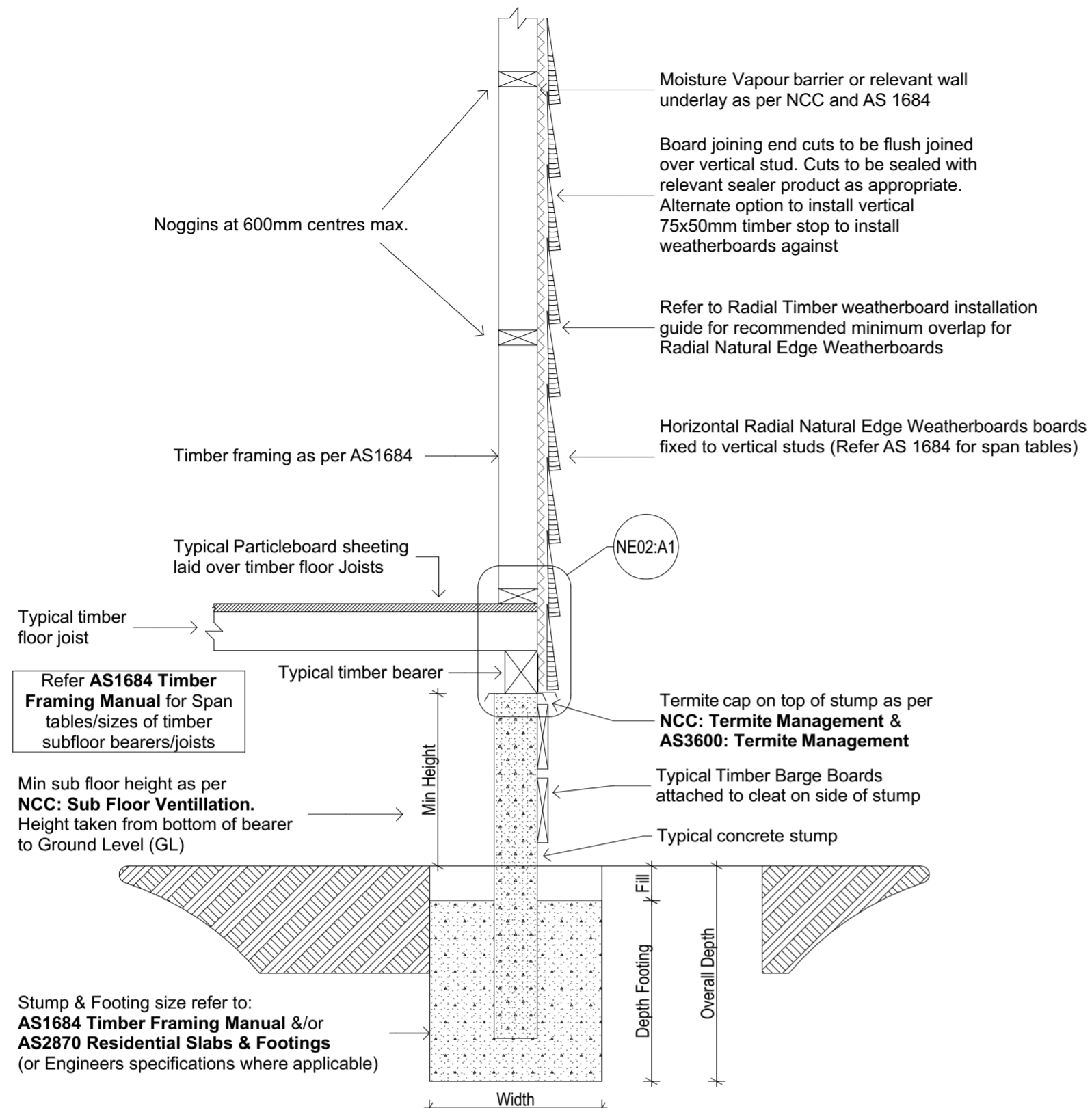
1.0 NE02:A - Horizontal Radial Natural Edge Weatherboard - Stud Frame: Timber Sub-Floor
