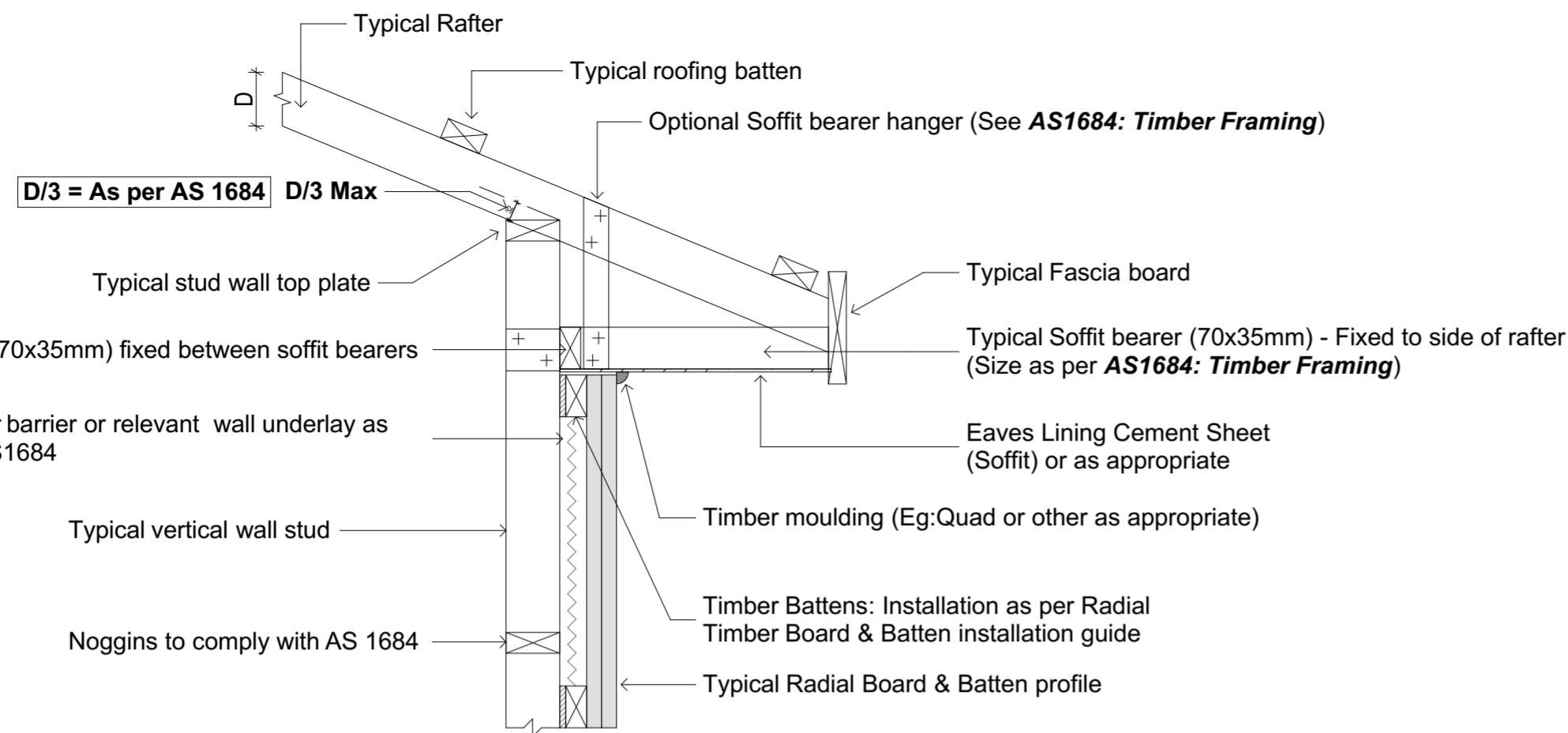
1.0 BB04:A - Typical Board & Batten Pitched Roof Detail Section (Batten Fixing)
