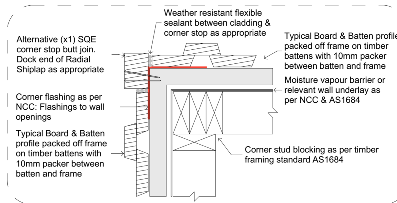
1.3 BB02:A2 - Board & Batten Alternate External Corner Details
