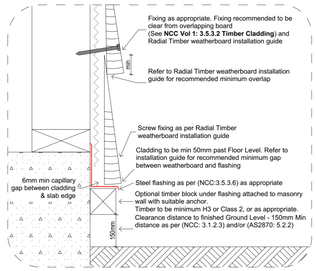
2.1 NE02:B1 - Radial Natural Edge Weatherboard SOG - Bottom Flashing
