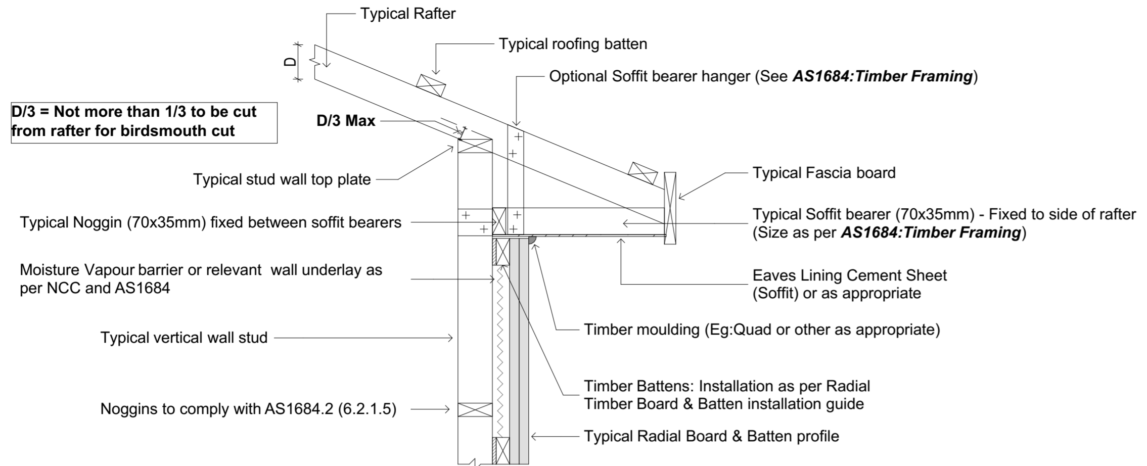
1.0 BB04:A - Typical Board & Batten Pitched Roof Detail Section (Batten Fixing)
