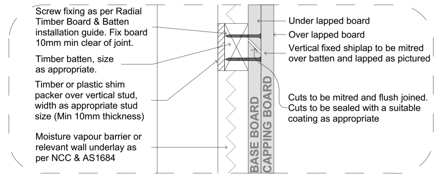
2.0 Typical Vertical B&B Mitre Join
