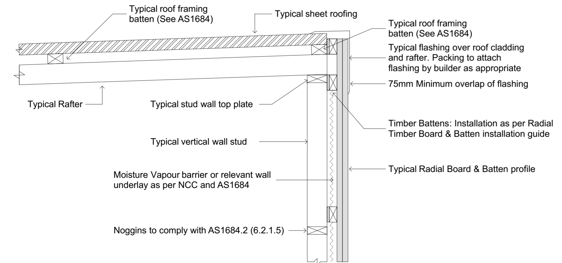
3.0 BB04:B - Typical Board & Batten Skillion Roof Detail Section (Batten Fixing)
