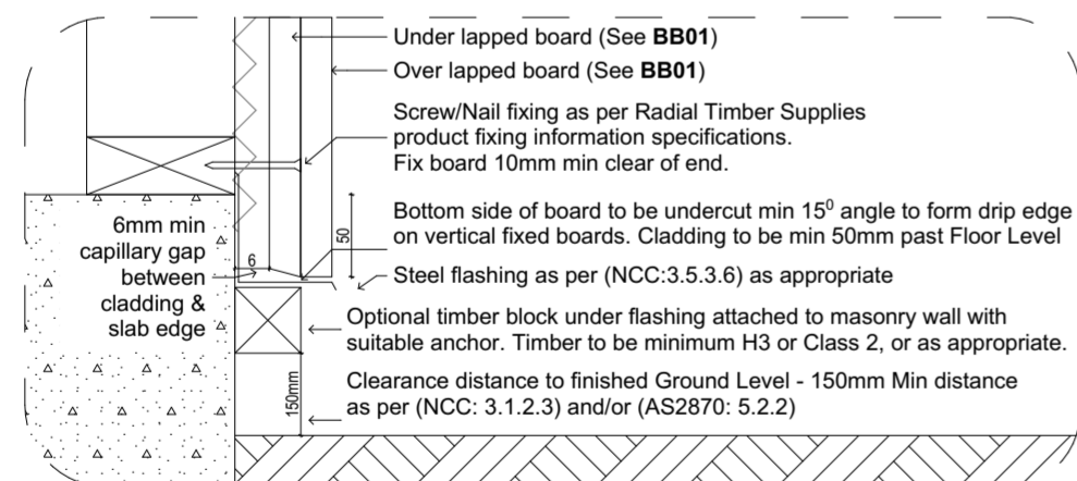
1.2 BB02:A2 - Vertical Board & Batten Bottom Flashing 1:5
