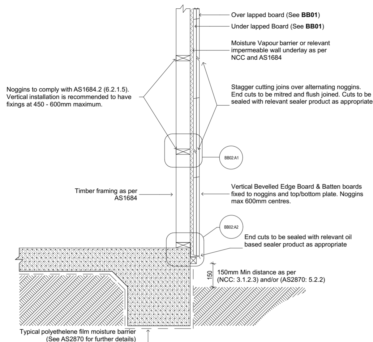
1.0 BB02:A - BE Board & Batten Noggin Fixing SOG 1:15
