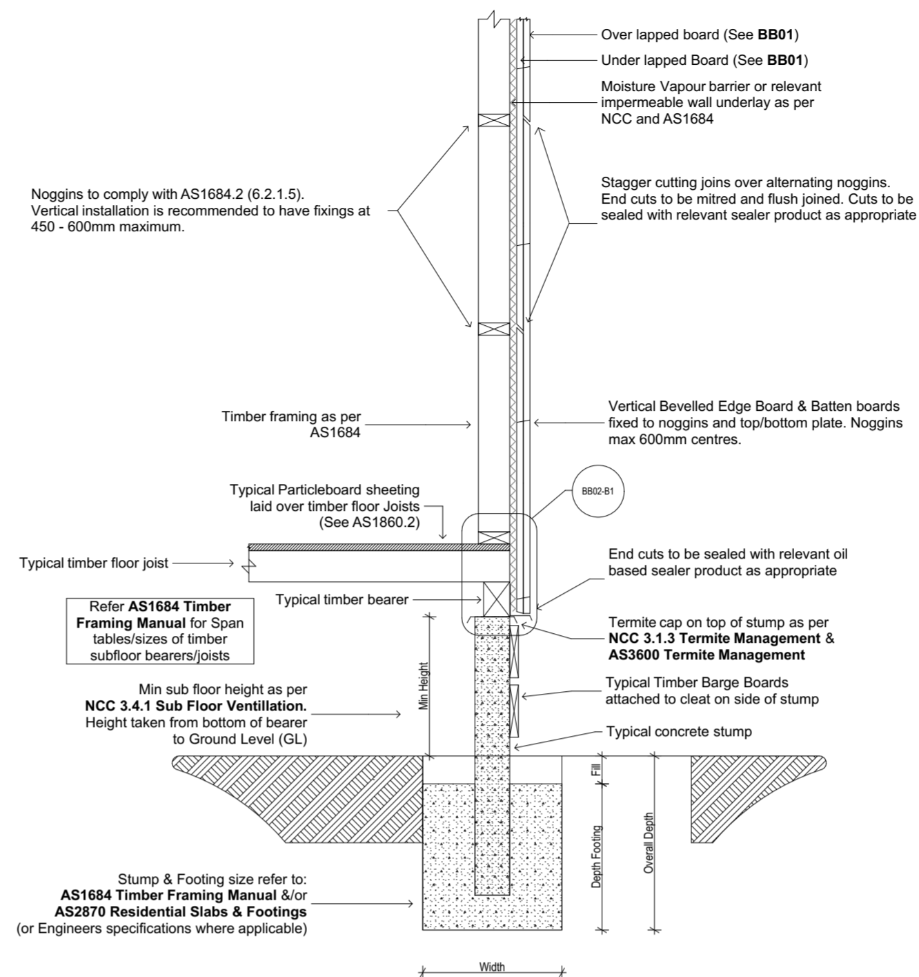
2.0 BB02:B - BE Board & Batten Noggin Fixing Timber Sub-Floor 1:15
