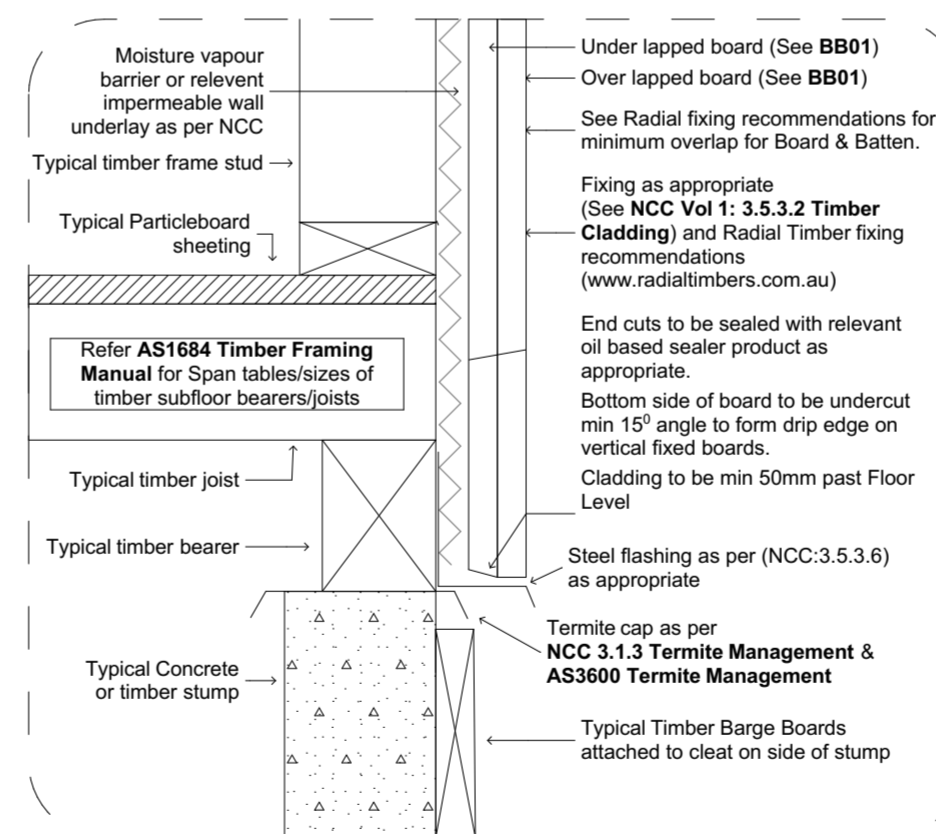
2.1 BB02:B1 - Vertical Board & Batten Bottom Flashing 1:5
