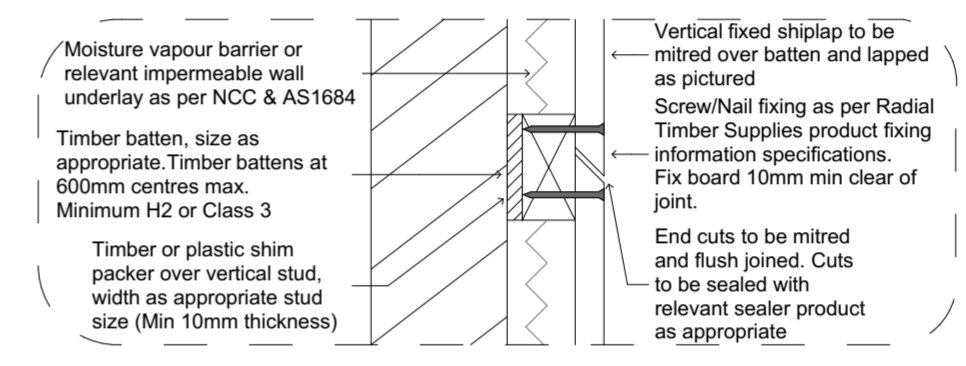
2.1 S03:A1 - Vertical Shiplap Mitre Join 1:5
