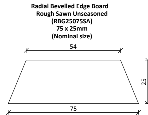
Radial BE (Bevelled Edge)(Pictured Left) Unseasoned Rough Sawn - Silvertop Ash: 50x23mm (Top) 75x25mm (Middle) 100x25mm (Bottom)
