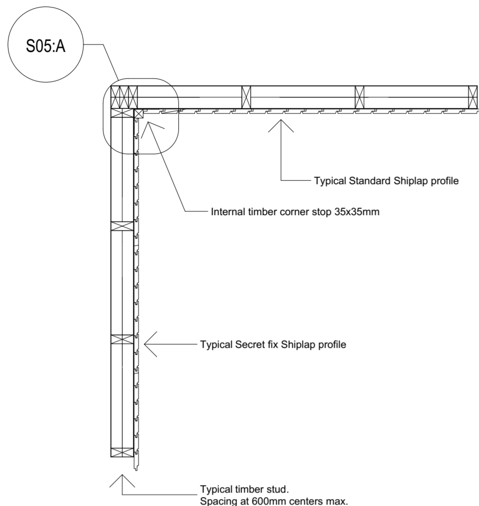
1.0 S05:A - Typical Radial Shiplap Internal Wall Corner Fixing Details: Plan View 1:15
