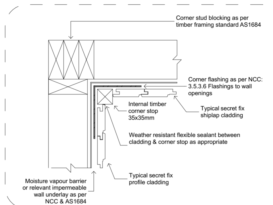
1.1 S05:A1 - Typical Radial Shiplap Internal Wall Corner Fixing Details 1:5
