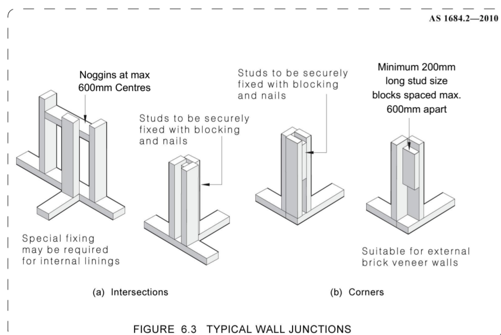
FIGURE 6.3 TYPICAL WALL JUNCTIONS
