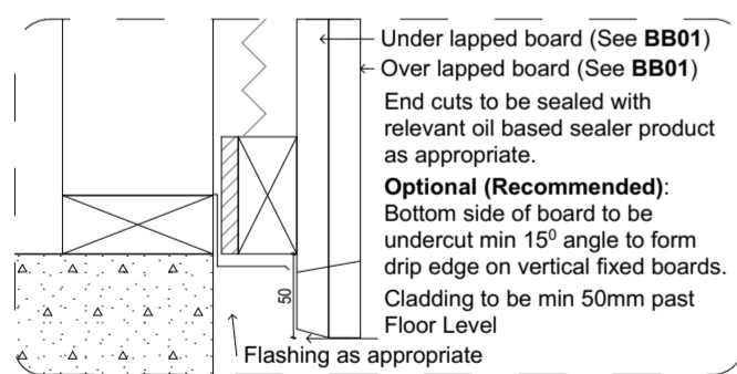
1.2 BB03:A2 - Vertical Board & Batten End Flashing 1:5
