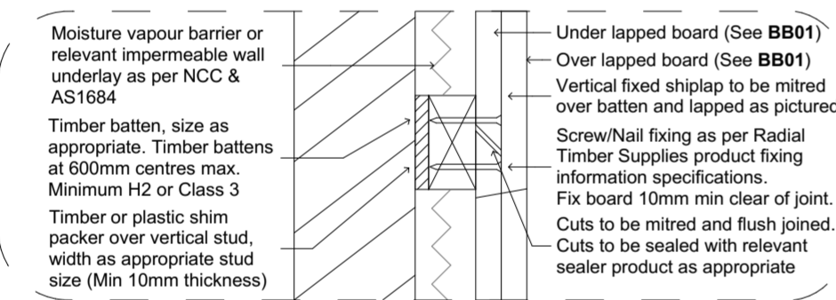
1.1/2.1 BB03:A1 & BB03:B1 - Vertical B&B Mitre Join 1:5
