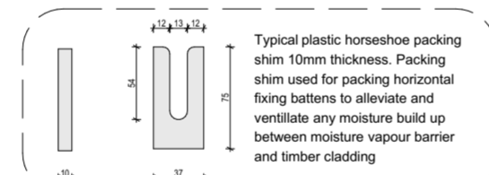
3.0 Typical Plastic Packer 1:5
