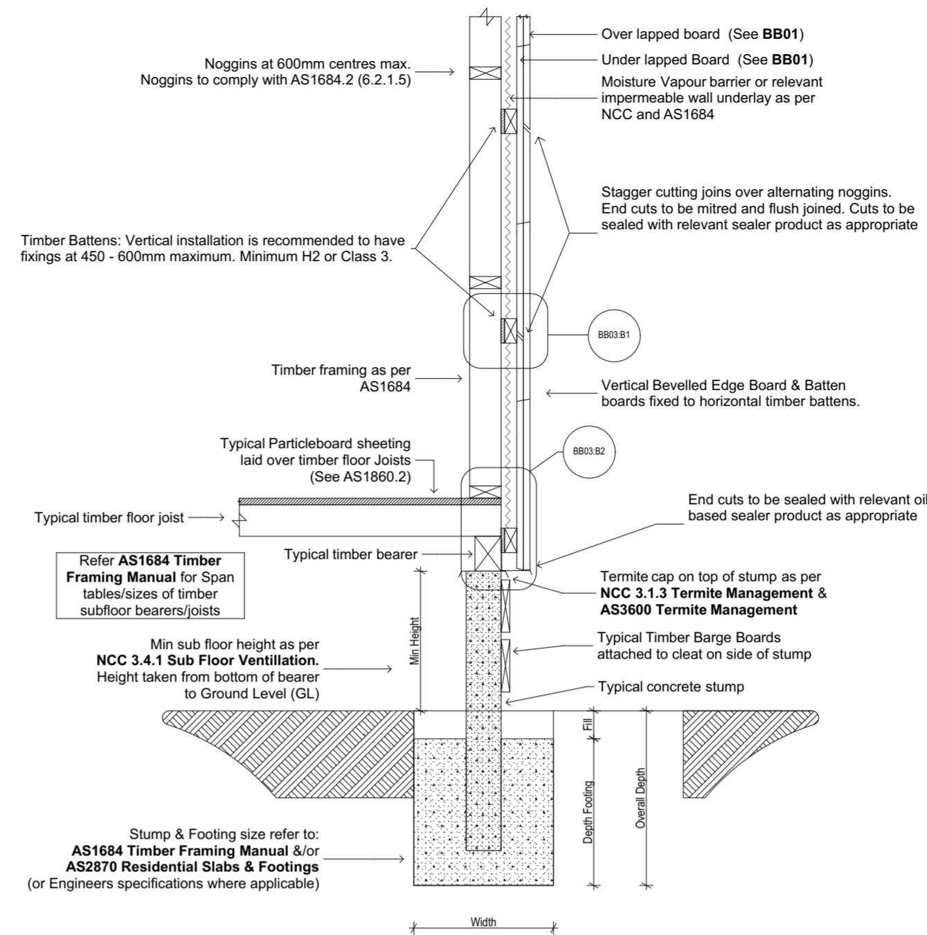
2.0 BB03:B - BE Board & Batten Batten Fixing Timber Sub-Floor 1:15
