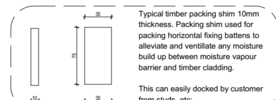
4.0 Typical Timber Packer 1:5
