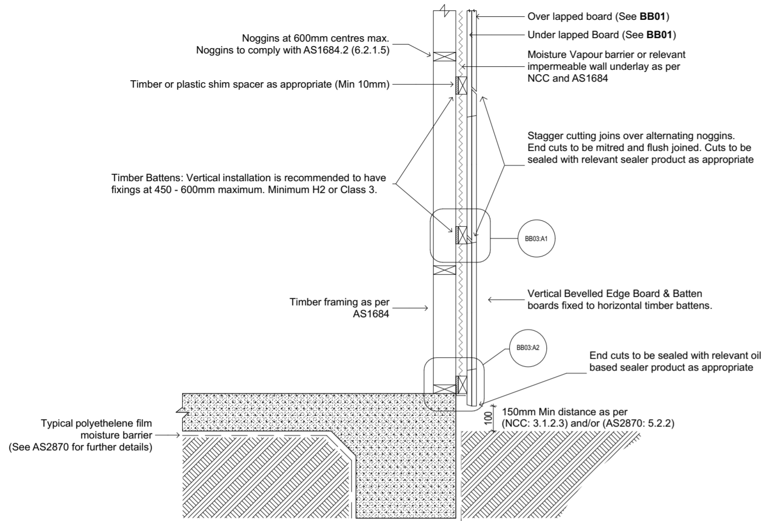
1.0 BB03:A - BE Board & Batten Batten Fixing SOG 1:15
