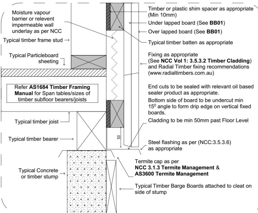
2.2 BB03:B2 - Vertical Board & Batten End Flashing 1:5
